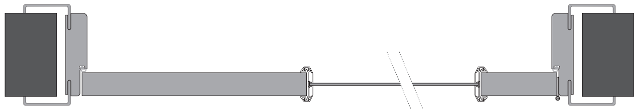
Section Of Glazed Interior Doors Mounted on the Wall (ex: 100G, 140G,...)
