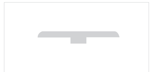
T-Molding Profile Section Produced from 6 mm MDF Panel.
